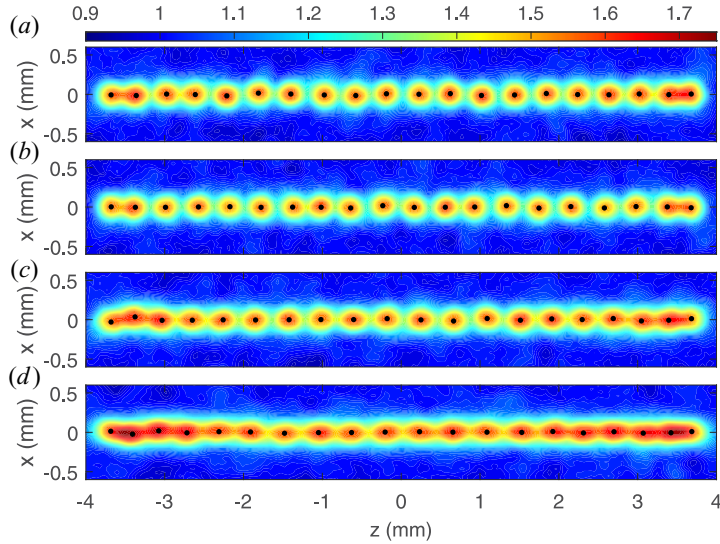
FIGURE 7. Final equilibrium ion density, where the colourbar indicates the density in units of the background density n_i/n_{i0} , n_{i0} = 2.1 \times 10^{14} \text{ m}^{-3} . The ion densities are shown for a slice through the xz plane averaged over 20 polarity cycles (40 ms). (a) Case 1, (b) Case 2, (c) Case 3 and (d) Case 4.
