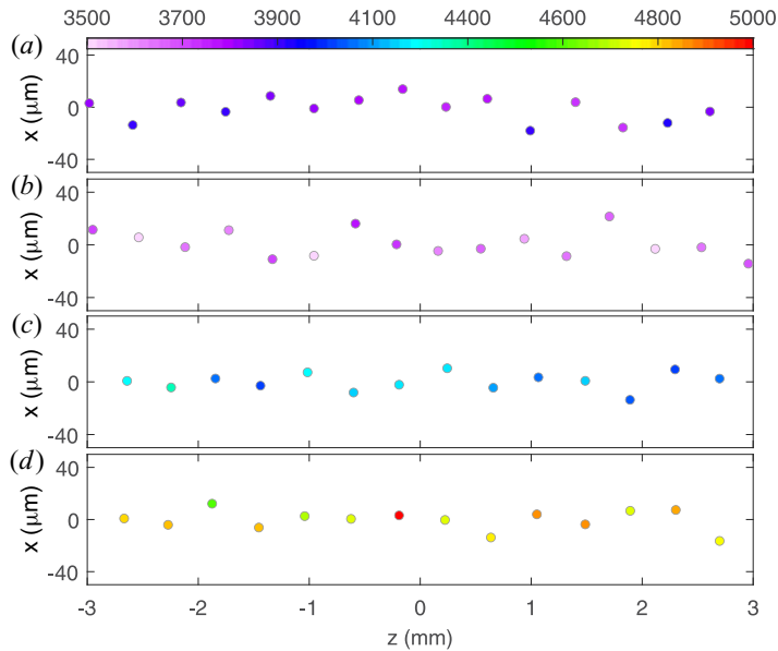
FIGURE 5. Final equilibrium charge and dust configuration for each case. Note that the scale in x is magnified to show the displacement from the central axis. The colour bar indicates the charge in units of elementary charge e^- . (a) Case 1; \langle Q_d \rangle = 3900e^- . (b) Case 2; \langle Q_d \rangle = 3670e^- . (c) Case 3; \langle Q_d \rangle = 4190e^- . (d) Case 4; \langle Q_d \rangle = 4820e^- .
