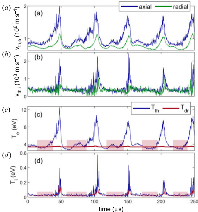
FIGURE 4. (a,b) Thermal velocities for the electrons and ions in the axial (blue) and radial (green) directions calculated from the standard deviation of the velocity distribution. The velocities in the tangential direction (not shown) are similar to those in the radial direction. (c,d) Temperature of the electrons and ions calculated from the thermal velocities, (2.1) (blue line), and the average temperature between ionization waves plus the drift energy, (2.3) (red line). The shaded areas indicate the times between the ionization waves when the ions thermalize with the neutral gas.
