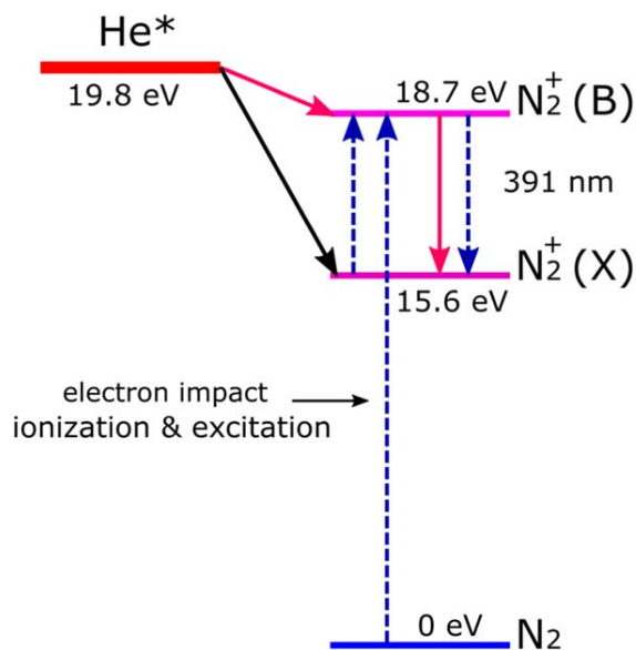
Figure 3. Simplified energy level diagram showing the dominant population pathways of the N_2^+(B) level. The dashed blue lines indicate pathways that are space and time dependent within the RF period, since they are induced by energetic electrons accelerated by the space and time dependent RF electric field. The solid lines indicate pathways, which are induced by heavy particle interactions between He metastables and nitrogen molecules (Penning ionization) and are space, but not (negligibly small) time modulated within the RF period.
