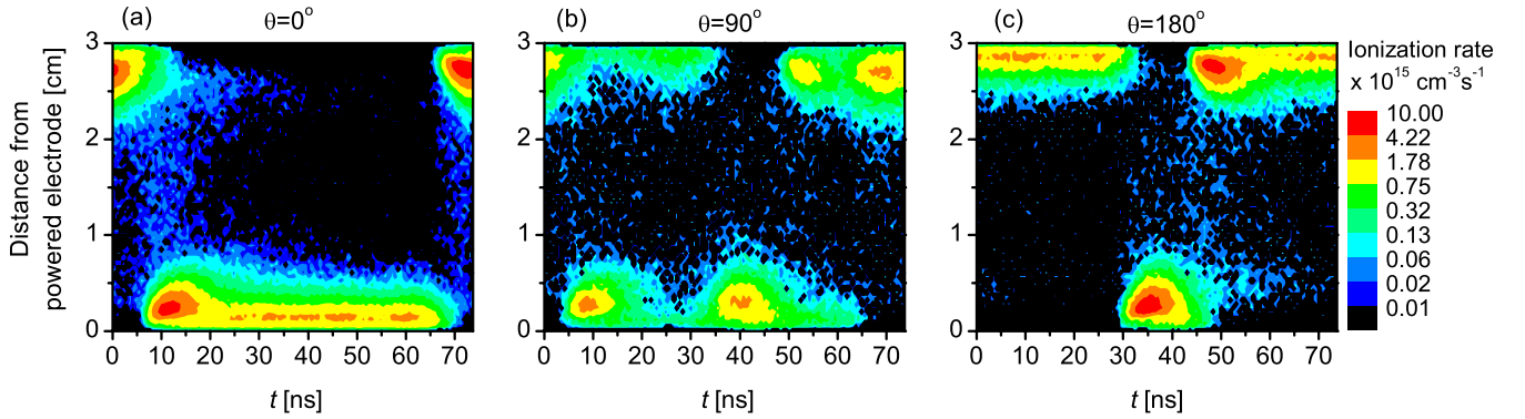
Figure 14. Spatio-temporal plots of the ionization rate for different values of \theta and N = 4 ( p = 100 \text{ Pa} , \phi_{tot} = 120 \text{ V} , \gamma = 0.4 ). The color scales are logarithmic.
